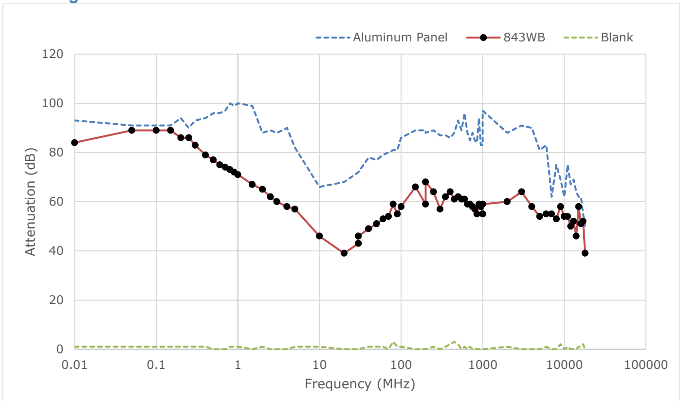
Figure 2. Attenuation of 843WB coating at different frequencies
